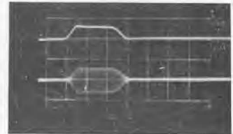
(Left) Amplitude modulation characteristic at 900 megacycles. Peak r-f output is 10 millivolts; r-f input, 50 millivolts. (Right) Oscillogram showing modulation pulse and r-f output pulse. Pulse duration is 0.25 \mu sec with .05 \mu sec rise time. Carrier frequency is 60 megacycles. Scale is 0.1 \mu sec per horizontal division.
