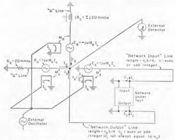
Schematic diagram of rf circuits of the Transfer-Function and Impittance Bridge.
