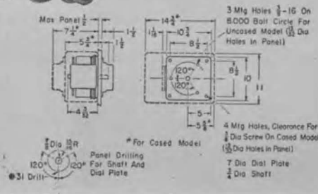
Types W30, W30M, W30H, and W30HM.
