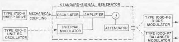
Figure 2. Modulation methods.
