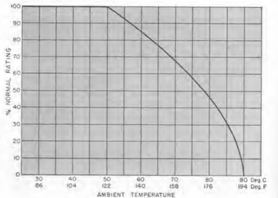
Figure 2. For ambient temperatures above 50 C, the unit should be derated according to this curve.
