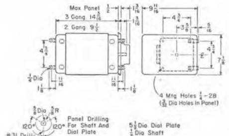
Ganged Types W10G2M, W10G3M, W10HG2M, W10HG3M (cased).
