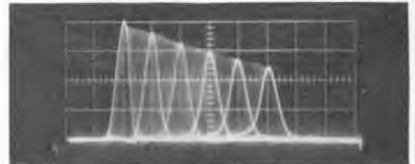
Oscillogram showing pulse shape and amplitude as delay setting is varied. Tektronix 541 Oscilloscope, 53K/54K Pre-Amplifiers; sweep, 0.1 \mu sec/cm.
