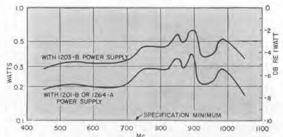
(Left) Typical pulse performance curves for the Type 1361-A UHF Oscillator with the Type 1264-A Power Supply. (Below) Typical curves of output vs. frequency for the Type 1361-A UHF Oscillator.
