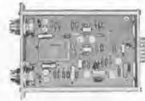
View of typical plug-in unit.
