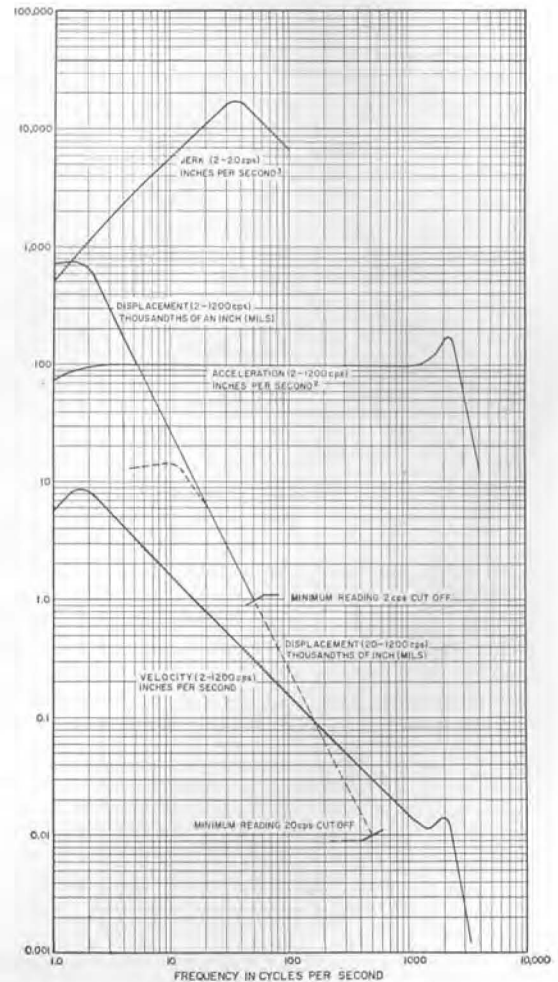
Readings of the Vibration Meter as a function of frequency for a constant acceleration of 100 inches per second 2 .
