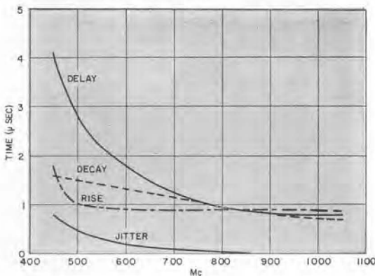
(Left) Typical pulse performance curves for the Type 1361-A UHF Oscillator with the Type 1264-A Power Supply. (Below) Typical curves of output vs. frequency for the Type 1361-A UHF Oscillator.
