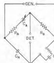
Figure 3. Four basic methods of obtaining resistance balance.
