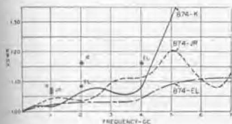
Typical VSWR of Types 874-K, -EL, and -JR. (Specifications are shown in red.)
