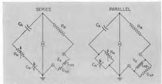
Elementary schematic of bridge configuration for series and parallel inductance measurement.
