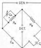
(Right) Figure 2. Circuits for capacitance bridges in which like reactances, C_N and C_P , or unlike reactances, L_A and C_P , are compared.
