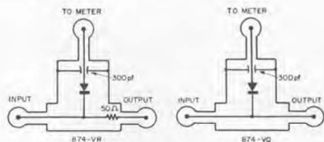
Schematic diagram of Types 874-VR and 874-VQ.
