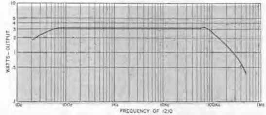
Output of the Type 1210-C Unit Oscillator with Type 1206-B Unit Amplifier, into 600-ohm load.
