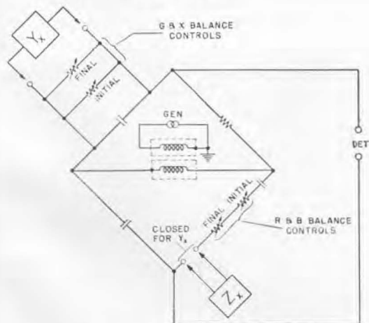
Elementary schematic diagram of the Type 1603-A Z-Y Bridge.
