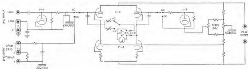
Elementary schematic diagram for the Type 1800-B Vacuum-Tube Voltmeter.
