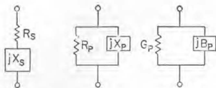
Figure 5. Series and parallel components of impedance.
