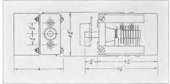
Over-all dimensions of TYPES 380-L, -M, and -N Decade-Condenser Units; dimension A is 3 3/16 inches. While TYPE 380-F uses the same switch mechanism, condensers are mounted on both sides of the switch and the panel space required is 4 3/4 x 4 1/4 inches.
