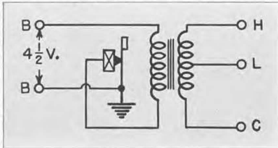
Schematic wiring diagram of the microphone hummer.
