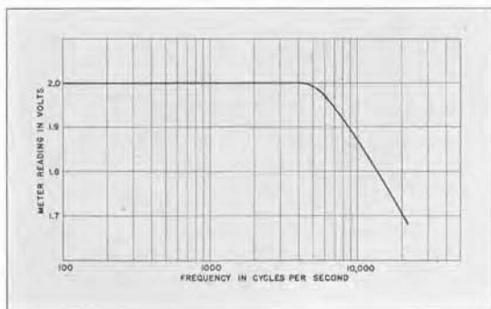
Average frequency characteristic of the meter.
