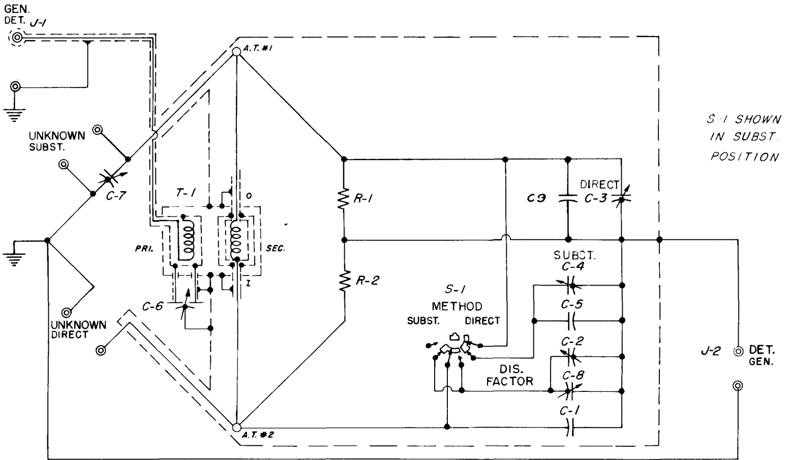
Wiring Diagram for Type 716-CS1 Capacitance Bridge
