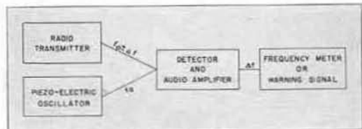
FIGURE 8. General functional diagram of a frequency monitoring system. The difference in frequency \Delta f between transmitter and piezo-electric oscillator is obtained in the detector, is amplified, and operates the frequency meter. To overcome ambiguity as to the sense of the deviation, \Delta f is made to have a definite value, say 1000 cycles, when the transmitter is at correct frequency, by adjusting the piezo-electric oscillator for a frequency 1000 cycles above or below the assigned transmitter frequency.
