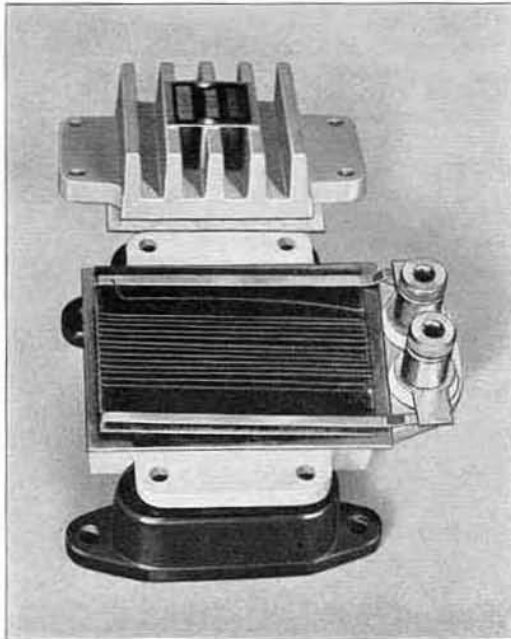
Photograph of TYPE 525-D Resistor with upper casting removed, showing construction of the resistance card.
