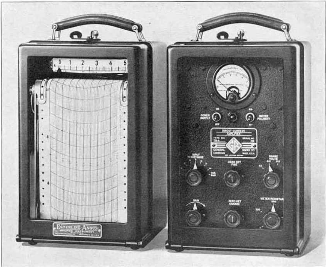
Esterline-Angus Recorder.
