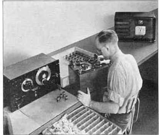
Measuring radio-receiver coils with the TYPE 721-A Coil Comparator.
