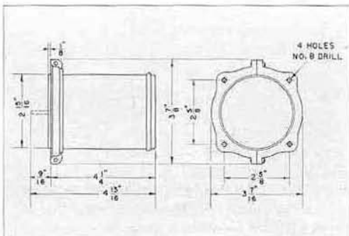
Dimensions of case for TYPE 641 Transformer.
