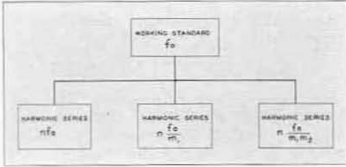
FIGURE 2. Showing functionally the operation of a frequency division system.
