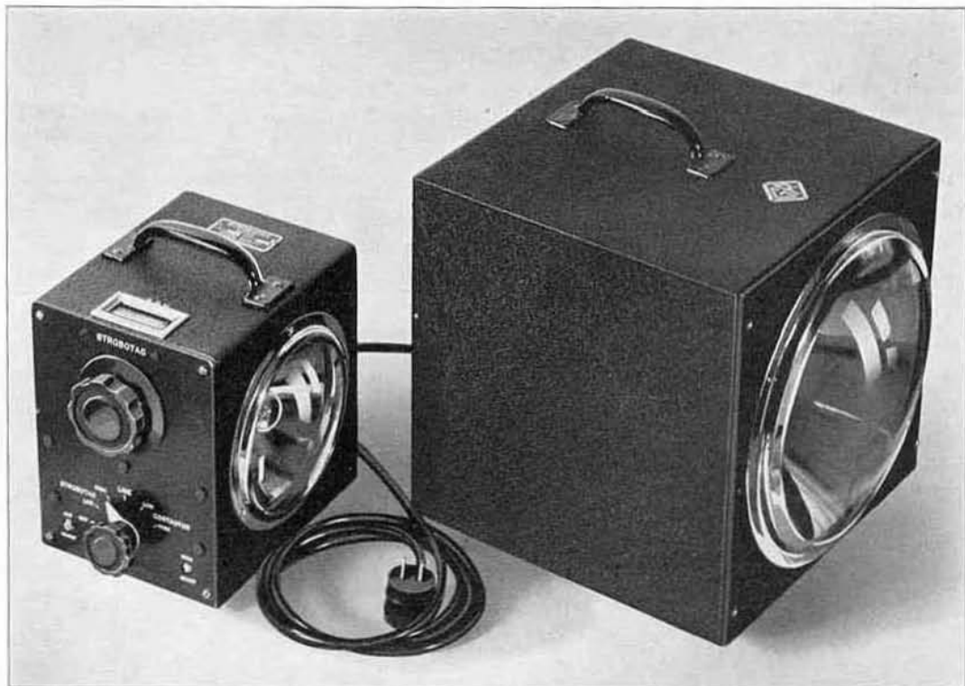
TYPE 631-B Strobotac and TYPE 648-A Stroboscope with connecting cables.
