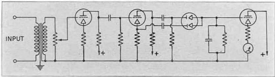
Schematic circuit diagram of the TYPE 686-A Power-Level Indicator.
