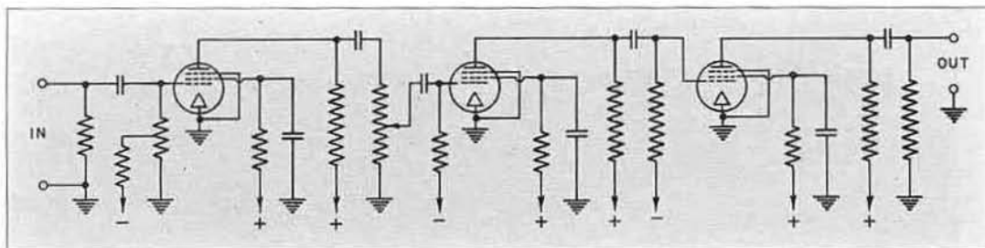
Schematic wiring diagram of TYPE 714-A Amplifier. Power supply and its filters are not shown.
