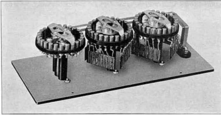
Interior of TYPE 670-F Compensated Decade Resistor.
