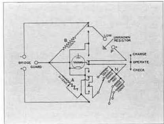
Schematic circuit diagram of the Megohm Bridge.
