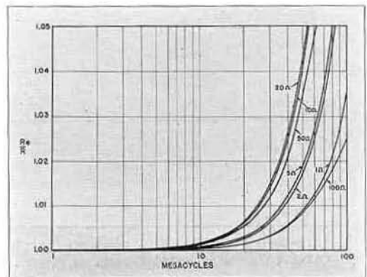
Ratio of effective resistance to d-c resistance as a function of frequency.
