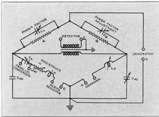
Schematic circuit diagram of the TYPE 516-C Radio-Frequency Bridge. By using the capacitance C_{PO} to balance the stray capacitance C_N , and the inductance L_D to balance the inductance L_N of the standard resistor, the bridge is made direct reading in both capacitance and resistance.
