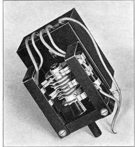
Rear View of TYPE 380-M.
