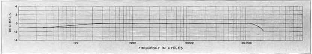
Frequency characteristic TYPE 741-P Plate-to-Line Transformer. Voltage step-down ratio 0.35:1.
