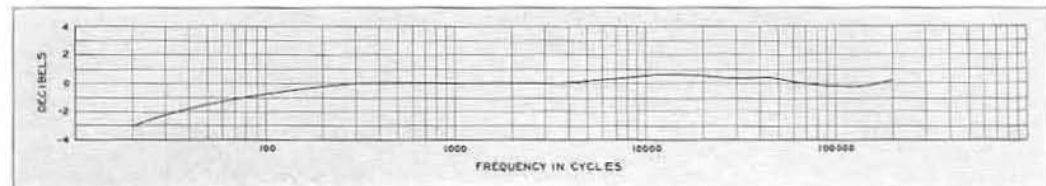
Frequency characteristic TYPE 741-G Line-to-Grid Transformer. Voltage step-up ratio 1:6.4.
