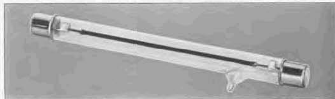
View of the high resistance standard used in TYPE 729-A Megohmmeter.
