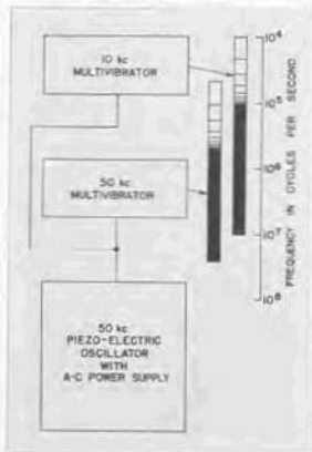
FIGURE 4. Functional diagram of CLASS C-10-11 Secondary Frequency Standard.
