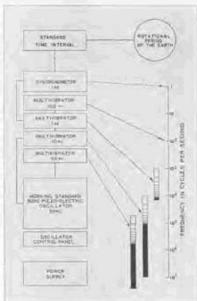
FIGURE 3. Functional diagram of CLASS C-21-4LD Primary Standard of Frequency. The output frequencies are shown in the spectra at the right of the diagram.
