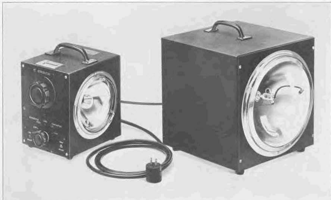
TYPE 631-B Strobotac with TYPE 648-A Strobolux.
