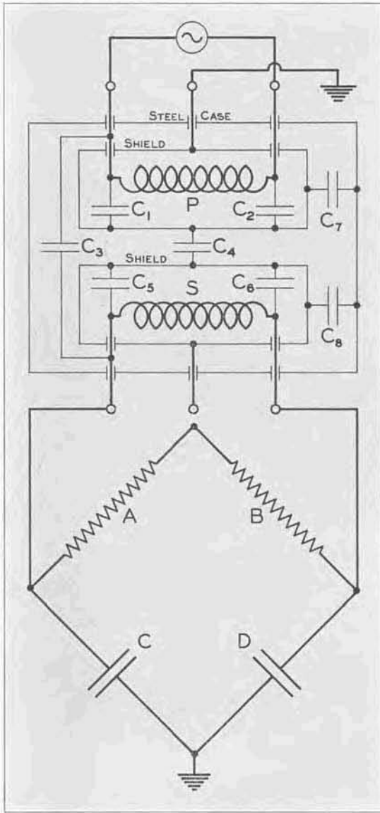
(Above) This diagram shows a grounded bridge supplied through a double-shielded transformer. When the case is grounded, the capacitance placed across each capacitance arm is 40 \mu\text{f} . This value is known and is considerably smaller than the unknown generator-to-ground capacitance which usually exists when a transformer is not used.
