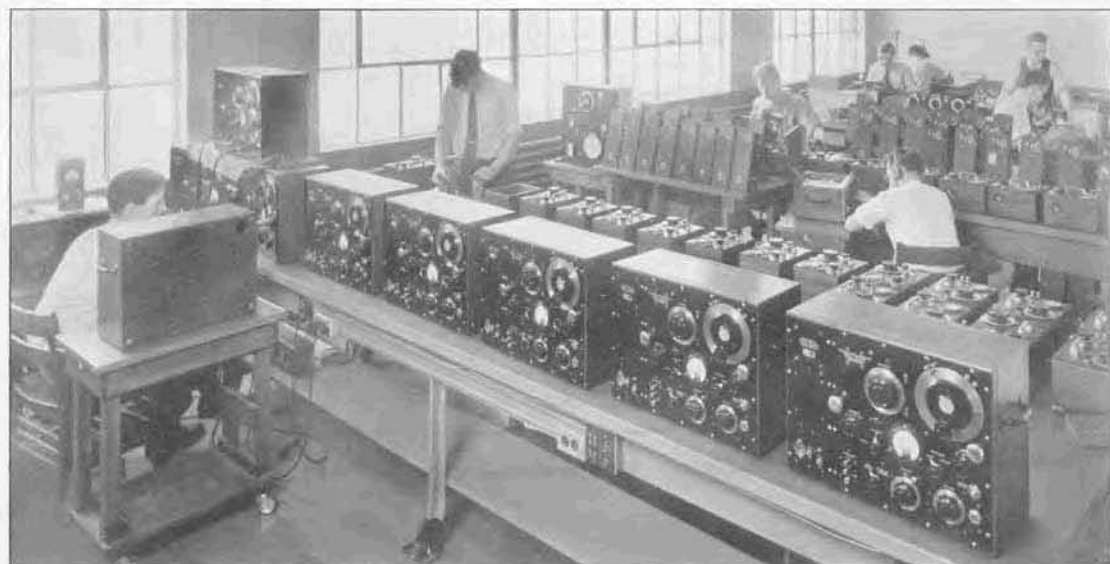
Calibrating and testing TYPE 605-B Standard-Signal Generators in the General Radio Standardizing Laboratory.
