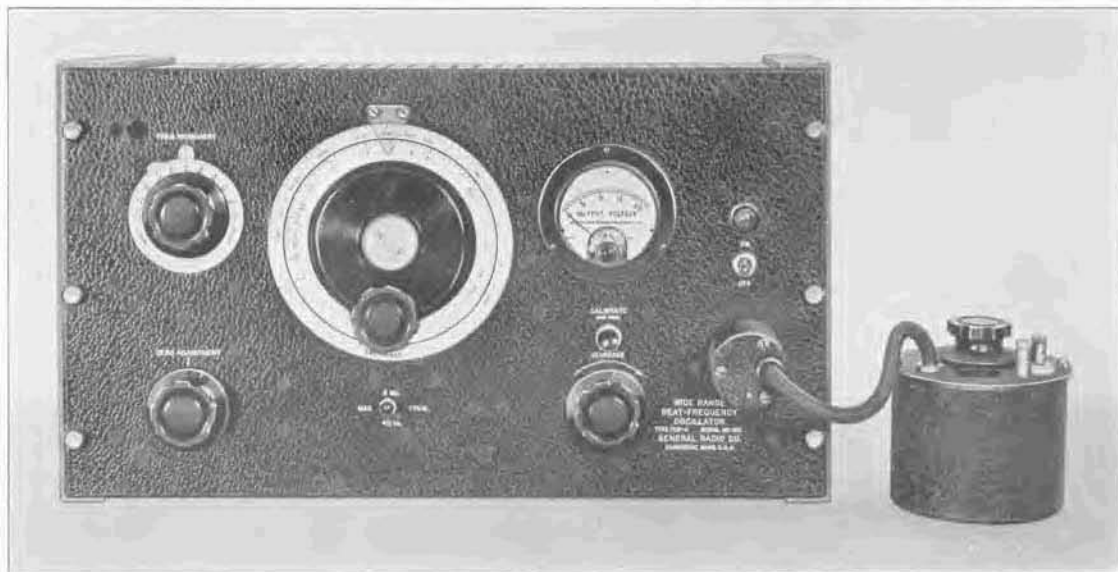
Panel view of TYPE 700-A Wide-Range Beat-Frequency Oscillator with TYPE 700-P1 Voltage Divider.
