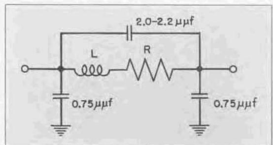
Equivalent circuit of TYPE 663 Resistor, mounted \frac{7}{8} inch above a metal panel.
