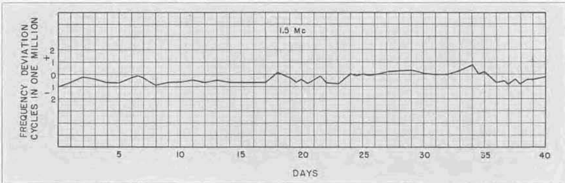
Record of the frequency of a stock TYPE 475-C Frequency Monitor operating at 1.5 Mc. Note that the deviation does not exceed ±1 cycle per million for the 40-day period.
