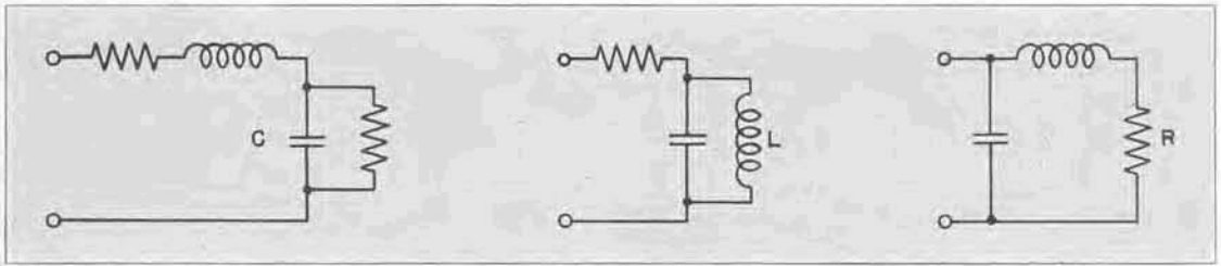
FIGURE 6. Schematic representation of capacitance, inductance, and resistance standards, showing the most important residual impedances. The ohmic resistance and inductance of the stacks and leads of the capacitor (left) are represented by series resistance and inductance, while the dielectric losses are represented by a shunt conductance. For an inductance (center), the copper losses and the distributed capacitance of the coil are the important residuals. A resistor (right), to a first approximation, is represented by an inductance in series, and a capacitance in shunt.
