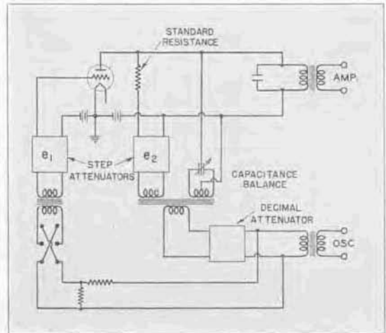
Simplified diagram of the circuit employed for the measurement of transconductance with the TYPE 561-D Vacuum-Tube Bridge. The a-c plate current resulting from the application of e_1 to the grid is balanced by an equal and opposite current applied to the plate from the source e_2 , through the standard resistance. The setting of the decimal attenuator at the bottom of the panel gives the significant figures in the result, and the settings of the step attenuators ( e_1 and e_2 ) indicate the multiplying factors (MULTIPLY BY and DIVIDE BY on the panel switches).
