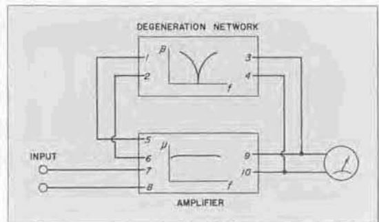
A functional diagram of the general type of circuit used in TYPE 760-A Sound Analyzer. The system consists of an amplifier with a propagation constant \mu and a feedback network with a propagation constant \beta having the frequency characteristics shown above. The degeneration network is highly selective, and at its null point the normal gain of the amplifier is obtained. At lower and higher frequencies, degeneration occurs, and the gain of the amplifier is greatly reduced.
