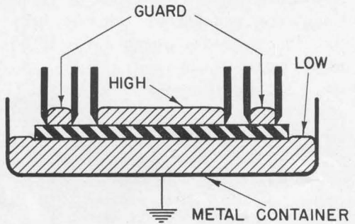
FIGURE 5. Cell for solid dielectrics, using mercury electrodes
