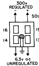
Figure 2-2. Power output connector. Both the 6.3-volt ac and the 300-volt dc supplies are isolated from ground to give greater latitude in external connections.
