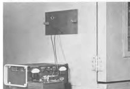
The built-in guard circuit permits the use of long leads from Comparator to sample inside conditioning chamber, as shown above.
