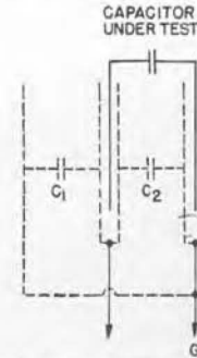
Sketch showing the nature and magnitude of the zero capacitance. This capacitance does not enter the measurement when a substitution method is used.
