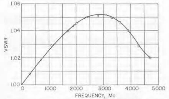
Standing-wave ratio of a typical TYPE 874-WM 50-ohm Termination as a function of frequency.
