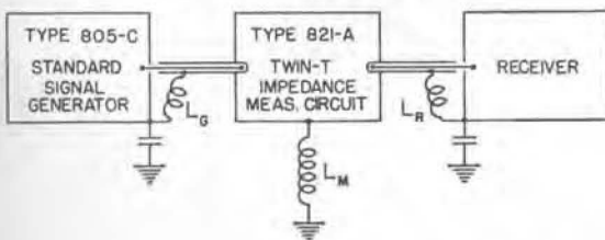
FIGURE 9. Showing how series inductance in the generator and detector leads can cause errors in measurement at radio frequencies.
