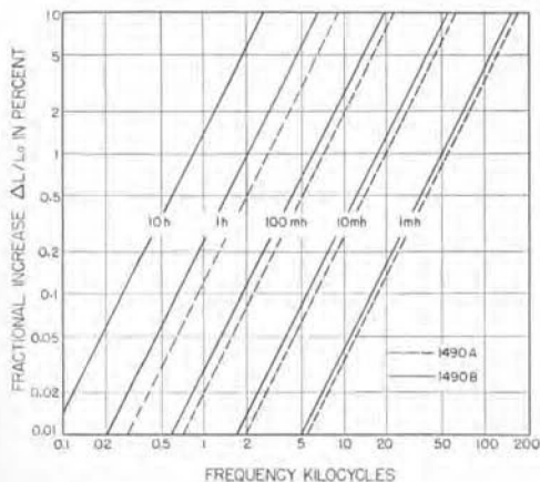
Percent increase in L_0 with frequency.
