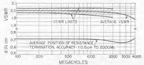
Plot of the VSWR and position of the pure resistance termination, for a Type 874-W100 100-Ohm Coaxial Standard. The distance, d, (see cross section above) is the distance from the position of the short or open circuit produced by a TYPE WN3 or WO3 Termination Unit to the position of the pure resistance termination. The cross-lined area indicates the tolerances on the characteristics.
