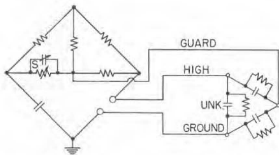
FIGURE 7. Elementary schematic circuit diagram of the TYPE 716-P4 Guard Circuit connected to the TYPE 716-C Capacitance Bridge showing the unknown capacitance and its terminal impedances.
