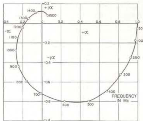
Plot of alpha versus frequency for a 1957 experimental, high-frequency transistor supplied by Bell Telephone Laboratories (Grounded base connection).
