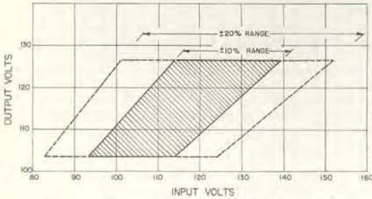
Range of operation for 115-volt models; for 230-volt models, multiply voltage scales by 2.
