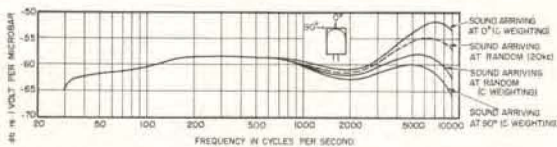
Typical response curves of TYPE 1551-B Sound-Level Meter with TYPE 759-P25 Dynamic Microphone Assembly.
