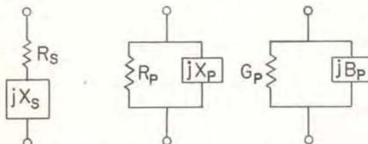
FIGURE 5. Series and parallel components of impedance.
