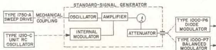
FIGURE 2. Modulation methods.
