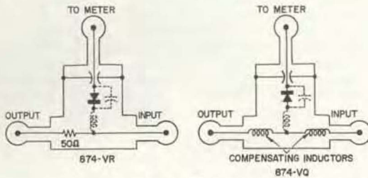
Schematics and average correction factor for TYPES 874-VR and -VQ.
