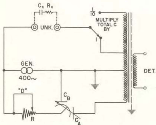
Schematic diagram of TYPE 1613-A Capacitance Bridge.
