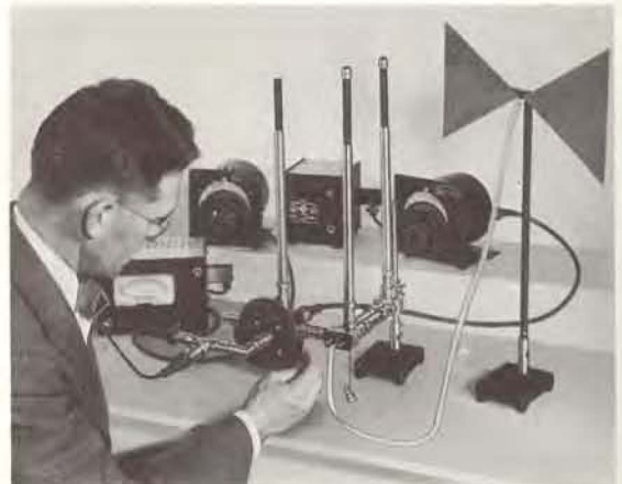
Figure 6. TYPE 874-Z Stands used to provide support for elements of a coaxial system.
