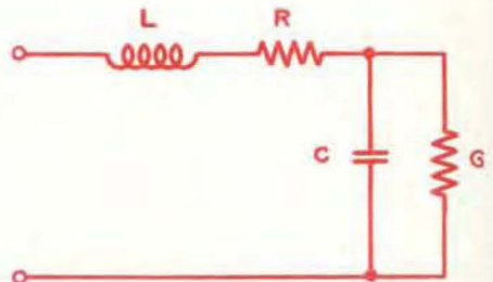
FIGURE 3. The equivalent circuit of a solid-dielectric capacitor.
