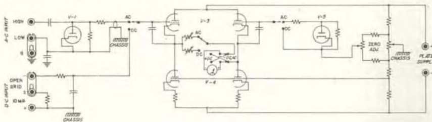
Elementary schematic circuit diagram for the TYPE 1800-B Vacuum-Tube Voltmeter.
