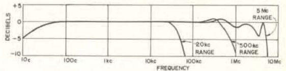
Typical Spectrum Level Characteristics for Type 1390-A Random-Noise Generator.
