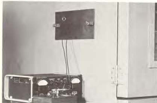
The built-in guard circuit permits the use of long leads from Comparator to sample inside conditioning chamber, as shown above.
