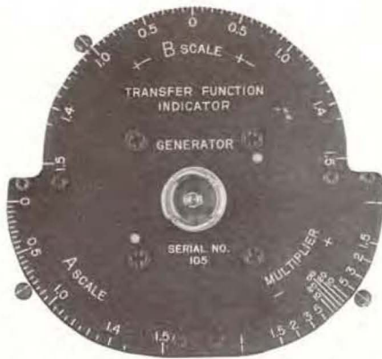
Dial calibrations of Transfer-Function Indicator (left) and Immittance Indicator (right).
