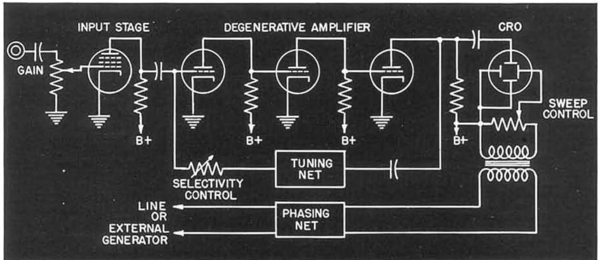
Schematic diagram for TYPE 707-A Cathode-Ray Null Detector.
