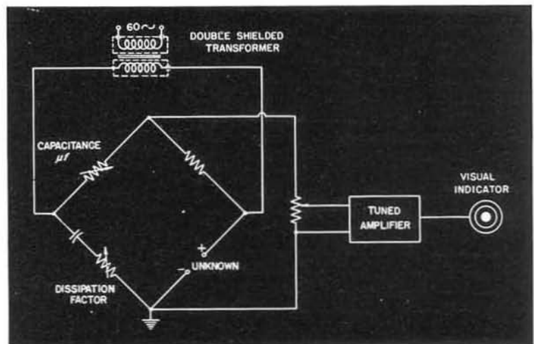
Schematic diagram of the TYPE 1611-A Capacitance Test Bridge. Generator and detector connections are interchanged by the switching when the bridge is used to measure capacitances greater than 1 \mu\text{f} .
