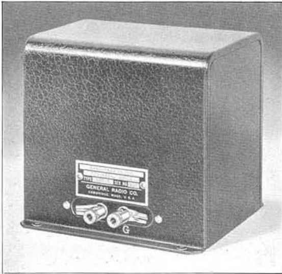
View of TYPE 530-A Filter.
