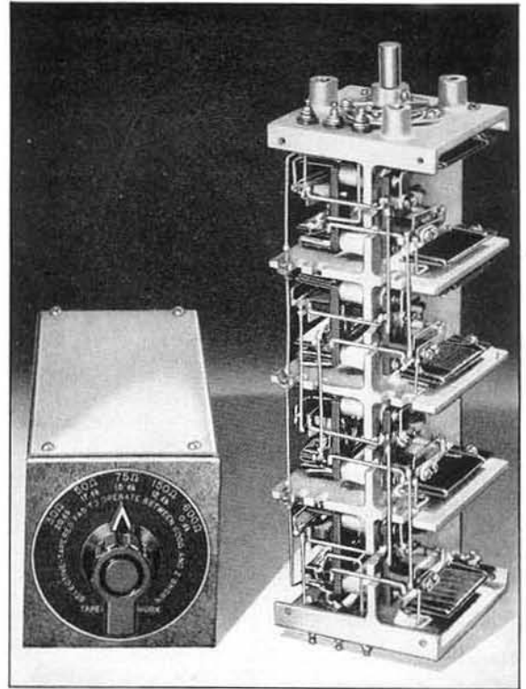
(Left) TYPE S29-HT Decade Attenuator Unit (tapered model), and (Right) typical internal construction of the TYPE S29 Decade Attenuator Units.
