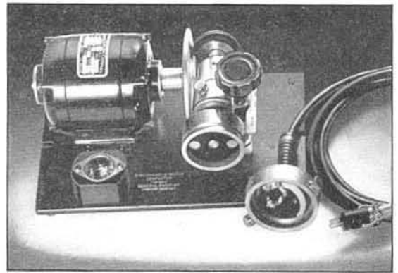
TYPE 549-C Synchronous-Motor-Driven Contactor.
