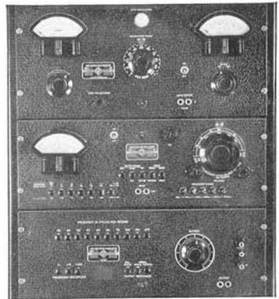
A relay-rack assembly of broadcasting test equipment showing, from top to bottom, TYPE 1931-A Amplitude-Modulation Monitor, TYPE 1932-A Distortion and Noise Meter, and TYPE 1301-A Low-Distortion Oscillator.
