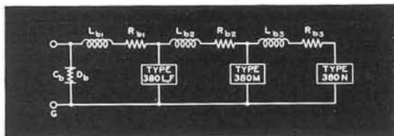
FIGURE 4. Equivalent circuit of a TYPE 219 Decade Condenser.
