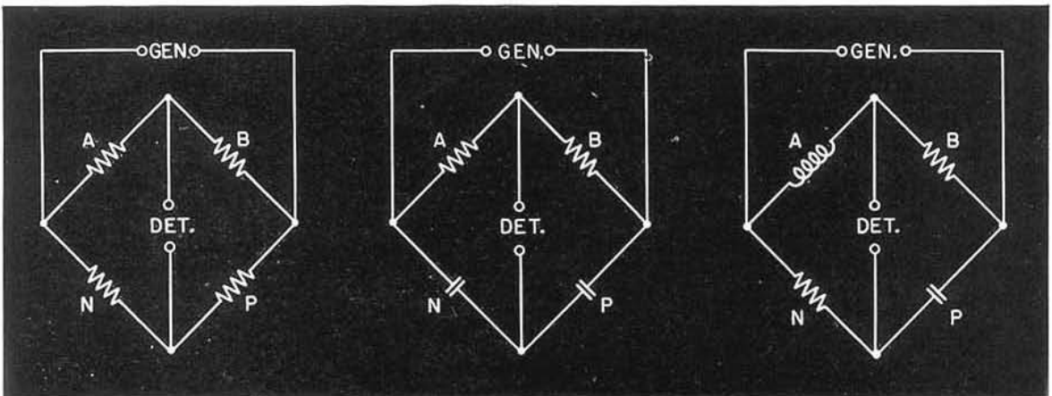
FIGURE 1. Left, the general Wheatstone bridge circuit; center, circuit for a capacitance bridge in which like reactances, N and P , are compared; and, right, a circuit in which unlike reactances, A and P , are compared.
