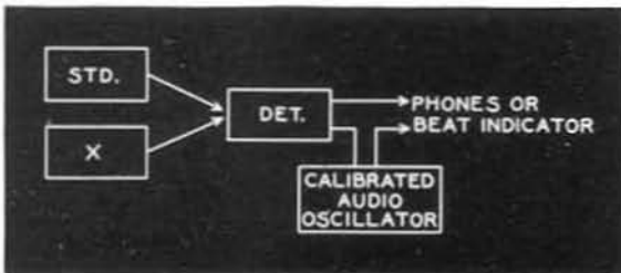
FIGURE 5. Functional diagram showing the operation of the direct-beating method of frequency measurement.
