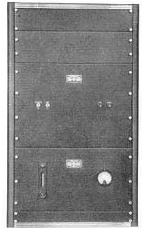
(Above) View of the TYPE 1100-AQ Secondary Frequency Standard. The cabinet rack is designed to be used on a table or bench. No synchronometer is included with this assembly, and a blank panel is supplied to fill the unused space at the top of the rack.
