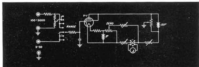
Elementary schematic diagram for TYPE 728-A D-C Vacuum-Tube Voltmeter.
