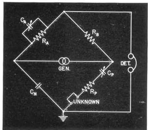
FIGURE 7. In the TYPE 916-A Radio-Frequency Bridge a series-substitution method of measurement is used. In this type of measurement stray capacitance to ground in the unknown arm can be particularly troublesome. Triple shielding is used in this arm to control the stray capacitances, as illustrated in Figure 8.
