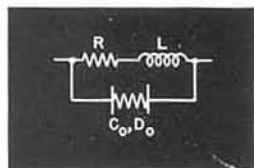
FIGURE 5. Equivalent circuit of an air-cored inductor L .
