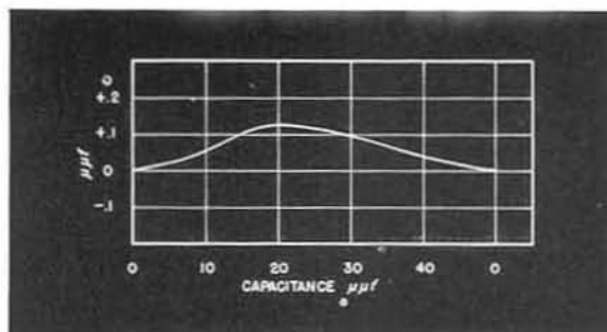
Plot of a typical worm correction for a TYPE 722 Precision Condenser.
