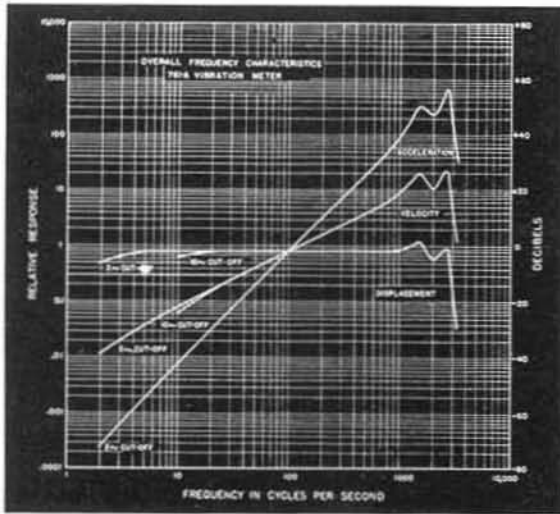
(Left) Over-all frequency characteristics of the vibration meter, including the vibration pickup.
