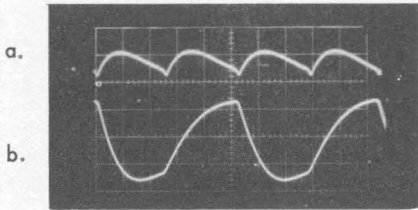
1-Mc Multivibrator - No trigger a. 0.2\mu\text{sec/cm} , 5.0 volts/cm. Junction D101, D102 b. 0.2\mu\text{sec/cm} , 10.0 volts/cm. TP3
