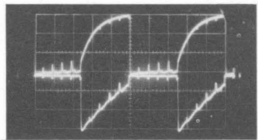
10-kc Multivibrator a. 20\mu\text{sec/cm} , 25 volts/cm. TP6 b. 20\mu\text{sec/cm} , 25 volts/cm. V105 pin 6
