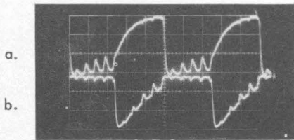
100-kc Multivibrator a. 2\mu\text{sec/cm} , 25 volts/cm. TP5 b. 2\mu\text{sec/cm} , 20 volts/cm. V104 pin 6
