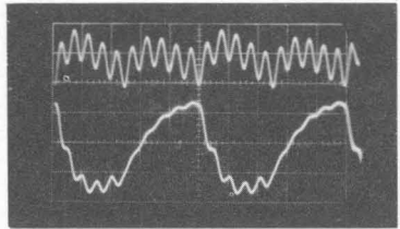
1-Mc Multivibrator - Triggered a. 0.2\mu\text{sec/cm} , 5.0 volts/cm. Junction D101, D102 b. 0.2\mu\text{sec/cm} , 10.0 volts/cm.
